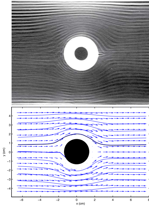
Fig. 9. Foam flow. Top: superimposed images evidence the streamlines (here from Fig. 1b). Bottom: measured velocity field and streamlines. The thicker solid line highlights the streamline analysed in Figure 10.
