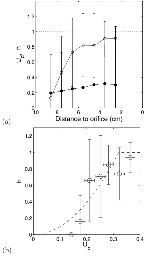
Fig. 17. Constriction: analysis of Figure 1c. (a) P_d/V_d (open circles) and U_d (closed circles) versus the distance to the constriction. (b) Plasticity fraction h estimated as h \approx P_d/V_d versus strain U_d (data from (a)): same figure as Figures 13 and 15, here with U_Y = 0.32 .
