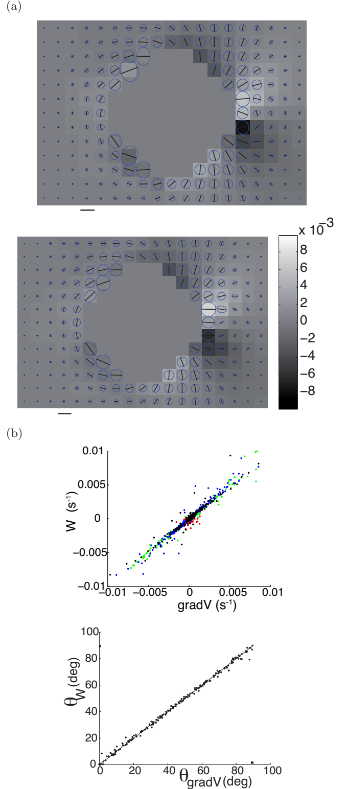
Fig. 3. Affine assumption: test of equation (8) on the foam of Figure 1b. (a) Comparison of maps of \mathbf{W} (top) and \nabla \mathbf{v} (bottom): ellipses, symmetric part; grey levels, antisymmetric part (bar: 5.6 \times 10^{-3} \text{ s}^{-1} ). (b) Quantitative comparison: top, (W_{XX} - W_{YY})/2 versus (\nabla v_{XX} - \nabla v_{YY})/2 , and the same for all other components (superimposed): XX + YY , XY - YX , XY + YX ; bottom, angle (in degrees) of ellipses plotted in (a). Each point comes from one RVE of the image.
