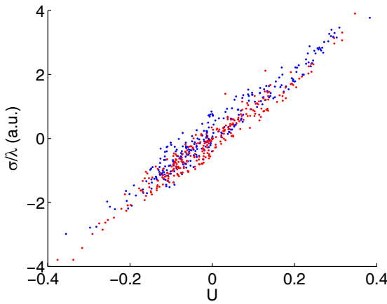
Fig. 4. XY components of the elastic stress \sigma (in arbitrary units) versus XY components of U . Each point comes from one RVE of the image of Figure 1b. The slope of the cloud of points is the foam's 2D shear modulus; it is of order of the bubbles' line tension \lambda to diameter ratio. Data for the (XX - YY)/2 components are superimposed: they have the same slope.
